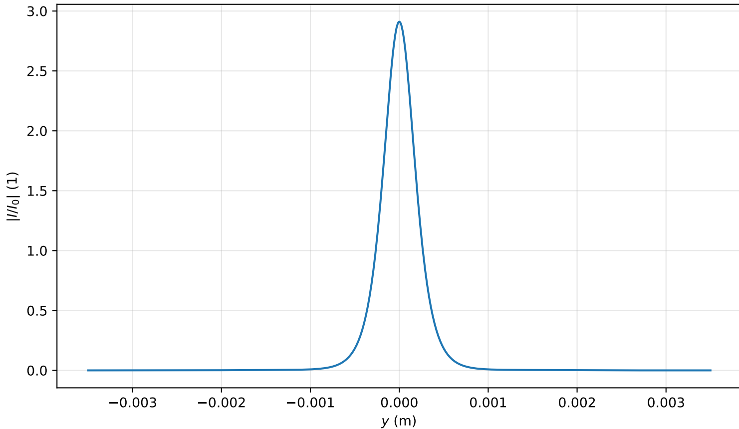
Intensity profile I(x=0, y, z=3.423)/I_0 , P_{in}=1.0P_{cr} , artificial time
